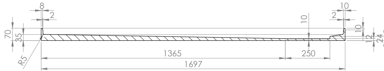
SECTION A-A CROSS SECTION VIEW
