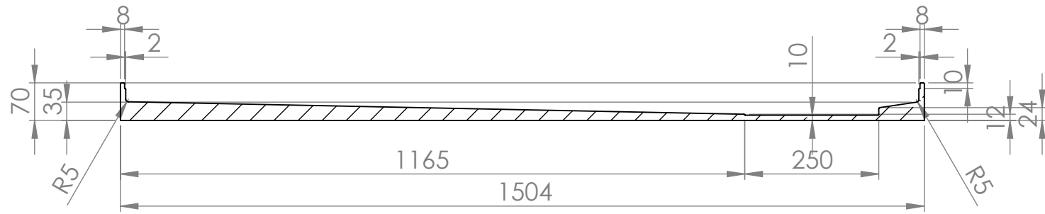
SECTION A-A CROSS SECTION VIEW
